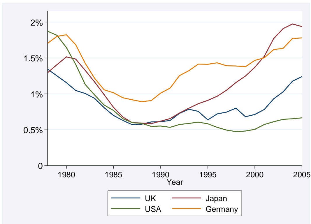
Figure 2: Share of climate-related innovation in UK and the top 3 inventing countries
